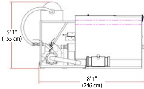
T30 HYDROSEEDER®
